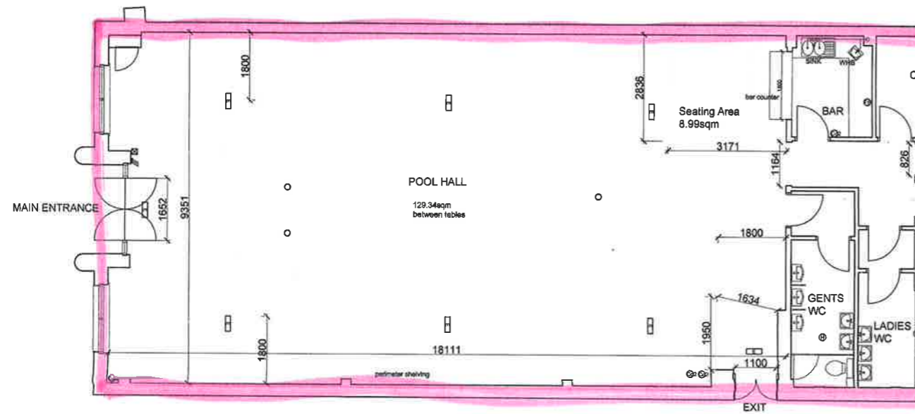
GROUND FLOOR PLAN AS PROPOSED 1:100
